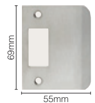
1301 Extended Strike to suit 1131 Latch (std +10mm)
