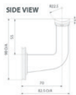
Showing flat mount adaptor
